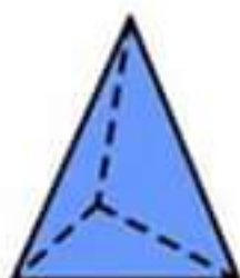
triangular pyramid
