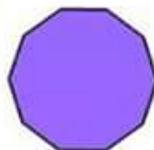
decagon
