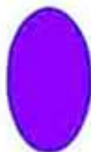
ELLIPSE
