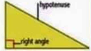
right triangle
